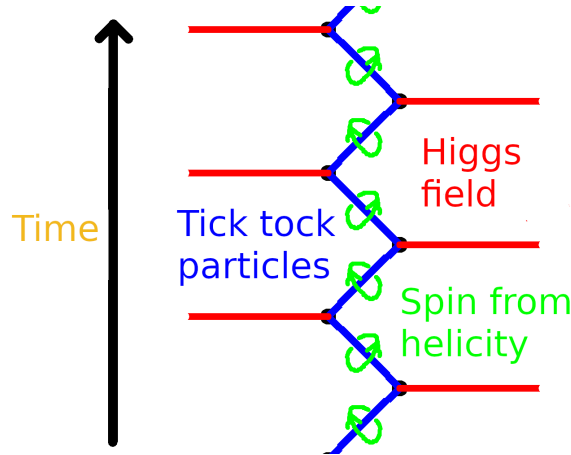
Figure 3: The tick-tock particle picture of the Dirac equation, after Penrose [38]. A massive electron (blue) alternates between right- and left-helicity massless segments, coupled at each vertex by the Higgs field (red). The green loops indicate spin emerging from the alternating helicity, the two \mathfrak{su}(2) factors of \mathfrak{so}(3,1) \cong \mathfrak{su}(2) \times \mathfrak{su}(2) made visual. Each vertex is a handoff event in the sense of Section 4.3: one quantum of action deposited, one helicity outcome recorded, one sample of proper time produced.
