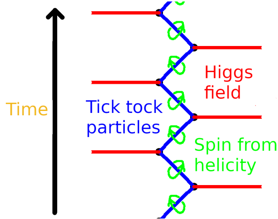
Figure 2: The tick-tock particle picture of the Dirac equation, after Penrose [39]. A massive electron (blue) alternates between right- and left-helicity massless segments, coupled at each vertex by the Higgs field (red). The green loops indicate spin emerging from the alternating helicity — the two \mathfrak{su}(2) factors of \mathfrak{so}(3, 1) \cong \mathfrak{su}(2) \times \mathfrak{su}(2) made visual. Each vertex is a handoff event in the sense of Section 4.3: one quantum of action deposited, one helicity outcome recorded, one sample of proper time produced.
