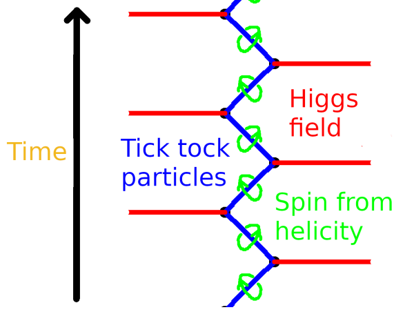
Figure 5: The tick-tock mechanism. A massive particle (blue) alternates between right- and left-helicity massless segments, coupled at each vertex by the Higgs field (red). Spin emerges from the alternating helicity flip at each vertex (green loops), visible as the two \mathfrak{su}(2) factors of \mathfrak{so}(3,1) \cong \mathfrak{su}(2) \times \mathfrak{su}(2) cycling between handoff events. Each vertex is a handoff event: one quantum of action deposited, one helicity outcome recorded, one sample of proper time produced.
