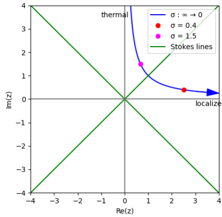
Figure 4: Trajectory of z = iq\sigma + \mu/\sigma in the complex plane as \sigma interpolates between the two limits of the Kraus family (14). The thermal limit \sigma \rightarrow \infty corresponds to z on the positive imaginary axis; the localized PVM limit \sigma \rightarrow 0 corresponds to z on the positive real axis. The green Stokes lines at \arg z = \pi/4 mark the boundary between the two asymptotic regimes of the parabolic cylinder function D_\nu(-z) , and therefore the boundary between the POVM and PVM descriptions of the transverse localization. Figure from [20].
