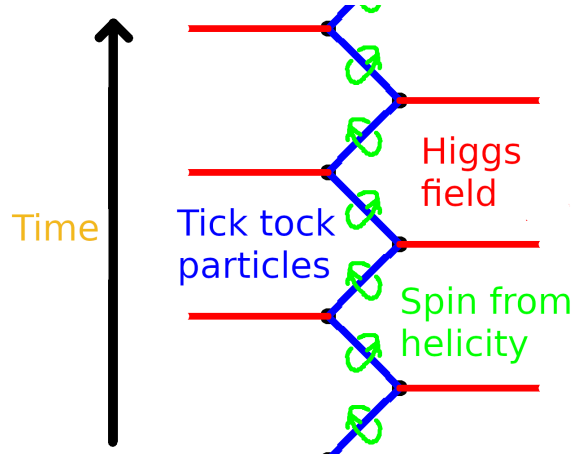
Figure 5: The tick-tock particle picture of the Dirac equation, after Penrose [38]. A massive electron (blue) alternates between right- and left-helicity massless segments, coupled at each vertex by the Higgs field (red). The green loops indicate spin emerging from the alternating helicity, the two \mathfrak{su}(2) factors of \mathfrak{so}(3,1) \cong \mathfrak{su}(2) \times \mathfrak{su}(2) made visual. Each vertex is a handoff event in the sense of Section 4.3: one quantum of action deposited, one helicity outcome recorded, one sample of proper time produced.
