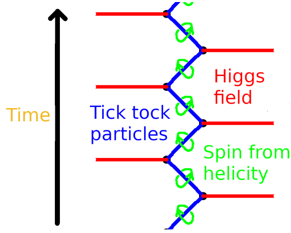
Figure 2: Adapted from [33]. Penrose's interpretation of the Dirac equation and the Higgs mechanism for an electron.
