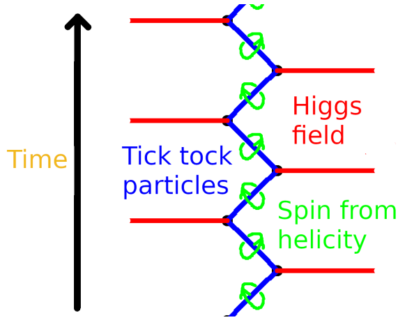
Figure 3: These figures were adapted from [21]. They show his interpretation of the Dirac equation and the Higgs mechanism for an electron.
