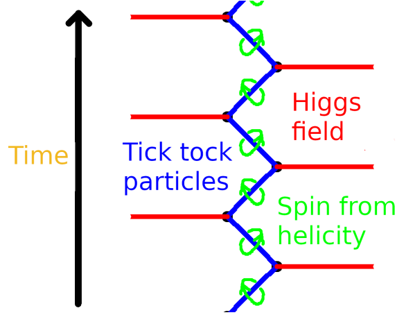
Figure 3: These figures were adapted from [18]. They show his interpretation of the Dirac equation and the Higgs mechanism for an electron.
