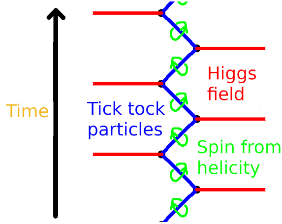
Figure 5: The tick-tock particle picture of the Dirac equation, after Penrose [40]. A massive electron (blue) alternates between right- and left-helicity massless segments, coupled at each vertex by the Higgs field (red). The green loops indicate spin emerging from the alternating helicity, the two \mathfrak{su}(2) factors of \mathfrak{so}(3,1) \cong \mathfrak{su}(2) \times \mathfrak{su}(2) made visual. Each vertex is a handoff event in the sense of Section 4.3: one quantum of action deposited, one helicity outcome recorded, one sample of proper time produced.
