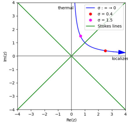
Figure 4: Trajectory of z = iq\sigma + \mu/\sigma in the complex plane as \sigma interpolates between the two limits of the Kraus family (16). The thermal limit \sigma \rightarrow \infty corresponds to z on the positive imaginary axis; the localized PVM limit \sigma \rightarrow 0 corresponds to z on the positive real axis. The green Stokes lines at \arg z = \pi/4 mark the boundary between the two asymptotic regimes of the parabolic cylinder function D_\nu(-z) , and therefore the boundary between the POVM and PVM descriptions of the transverse localization. Figure from [20].
