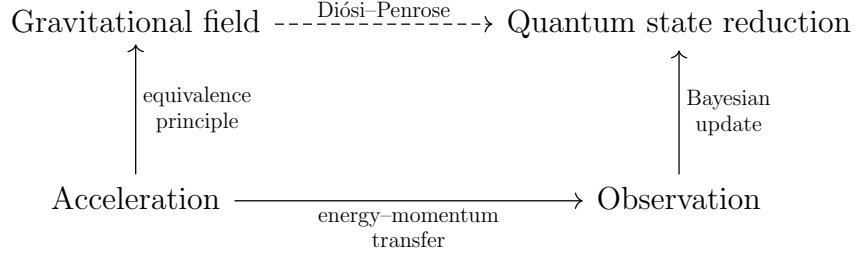
Figure 5: Solid arrows denote subjective grounding relations: A \rightarrow B means every instance of B is physically realized by an instance of A , for a given observer. The dashed arrow denotes the Diósi–Penrose postulate, where the relation is claimed to hold objectively rather than observer-relatively.
