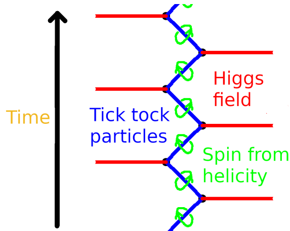
Figure 3: These figures were adapted from [20]. They show his interpretation of the Dirac equation and the Higgs mechanism for an electron.
