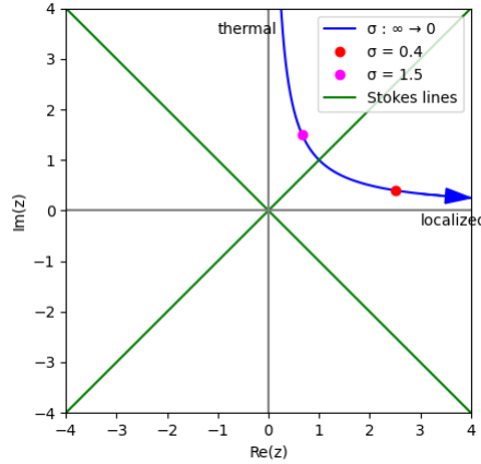
Figure 3: Trajectory of z = iq\sigma + \mu/\sigma in the complex plane as \sigma interpolates between the two limits of the Kraus family (15). The thermal limit \sigma \rightarrow \infty corresponds to z on the positive imaginary axis; the localized PVM limit \sigma \rightarrow 0 corresponds to z on the positive real axis. The green Stokes lines at \arg z = \pi/4 mark the boundary between the two asymptotic regimes of the parabolic cylinder function D_\nu(-z) , and therefore the boundary between the POVM and PVM descriptions of the transverse localization. Figure from [20].
