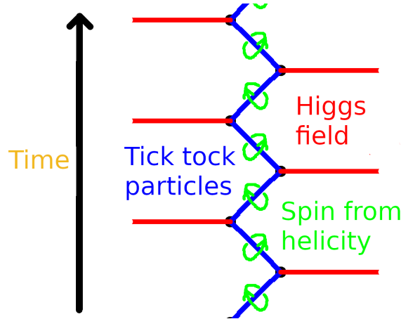
Figure 5: The tick-tock particle picture of the Dirac equation, after Penrose [38]. A massive electron (blue) alternates between right- and left-helicity massless segments, coupled at each vertex by the Higgs field (red). The green loops indicate spin emerging from the alternating helicity, the two \mathfrak{su}(2) factors of \mathfrak{so}(3,1) \cong \mathfrak{su}(2) \times \mathfrak{su}(2) made visual. Each vertex is a handoff event in the sense of Section 4.3: one quantum of action deposited, one helicity outcome recorded, one sample of proper time produced.
