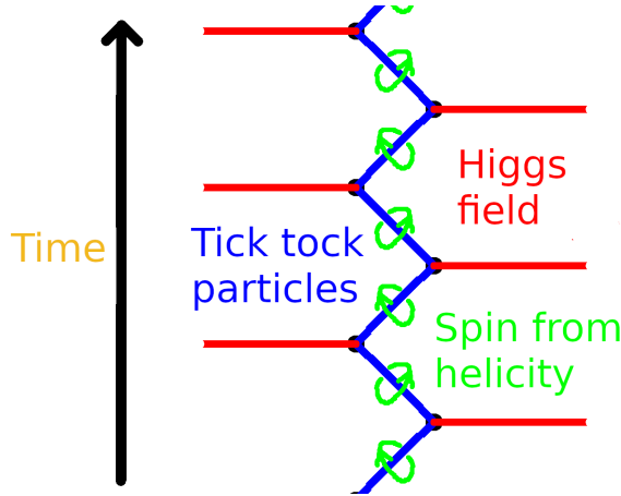
Figure 2: The tick-tock particle picture of the Dirac equation, after Penrose [33]. A massive electron (blue) alternates between right- and left-helicity massless segments, coupled at each vertex by the Higgs field (red). The green loops indicate spin emerging from the alternating helicity — the two \mathfrak{su}(2) factors of \mathfrak{so}(3,1) \cong \mathfrak{su}(2) \times \mathfrak{su}(2) made visual. Each vertex is a handoff event in the sense of Section 4.3: one quantum of action deposited, one helicity outcome recorded, one sample of proper time produced.
