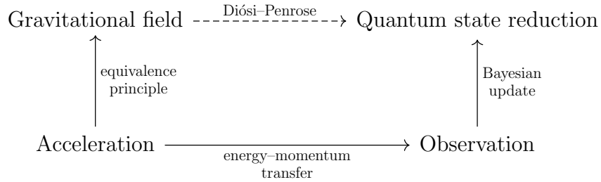
Figure 5: Solid arrows denote subjective grounding relations for a given observer: A \rightarrow B means every instance of B is physically realised by an instance of A . This paper establishes only the bottom and right solid arrows: proper acceleration produces energy–momentum transfer, and energy–momentum transfer underlies observation via Bayesian update. Together these give a subjective path from acceleration to quantum state reduction — measurement can source gravitational effects consistent with known thermodynamics. The dashed arrow is the Diósi–Penrose postulate, which claims the reverse direction holds objectively : gravitational self-interaction collapses the wavefunction. We do not adopt this arrow. The diagram is explicitly asymmetric, and that asymmetry is the point.
