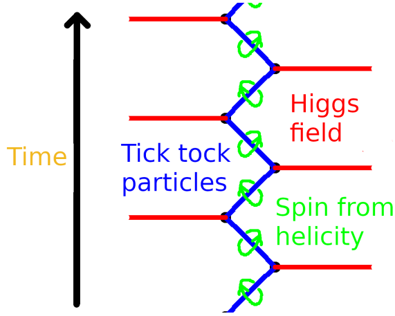
Figure 3: The tick-tock particle picture of the Dirac equation, after Penrose [36]. A massive electron (blue) alternates between right- and left-helicity massless segments, coupled at each vertex by the Higgs field (red). The green loops indicate spin emerging from the alternating helicity, the two \mathfrak{su}(2) factors of \mathfrak{so}(3, 1) \cong \mathfrak{su}(2) \times \mathfrak{su}(2) made visual. Each vertex is a handoff event in the sense of Section 4.3: one quantum of action deposited, one helicity outcome recorded, one sample of proper time produced.
