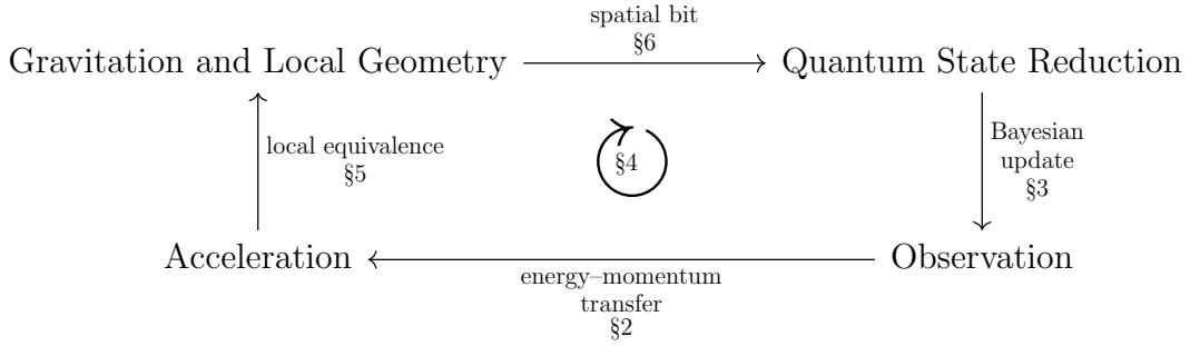
Figure 1: Arrows denote subjective grounding relations for a given observer: A \rightarrow B means every instance of A is physically realized by an instance of B . This paper explores the arrows. The Diósi–Penrose postulate says that gravitation triggers state reduction, while this paper constructs the converse for a specific example, that state reduction physically realizes local geometry.
