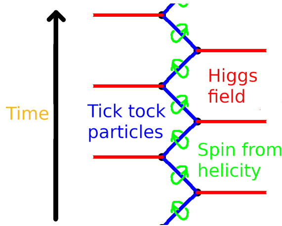
Figure 3: These figures were adapted from [18]. They show his interpretation of the Dirac equation and the Higgs mechanism for an electron.
