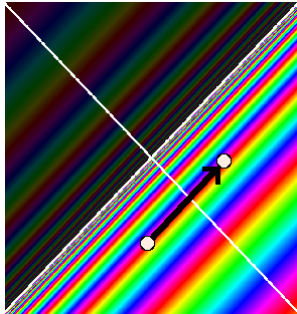
Figure 3: The points \mathcal{P} and \mathcal{R} are marked with white dots, connected by the null geodesic (black arrow). The rainbow coloring shows the Rindler mode frequency structure across the wedge. A PVM projection onto this null line selects a single frequency from the thermal superposition, replacing the full delocalized mode with the localized non-thermal microstate of equation (27).
