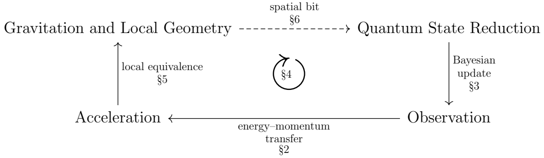
Figure 1: Solid arrows denote subjective grounding relations for a given observer: A \rightarrow B means every instance of A is physically realized by an instance of B . This paper explores the arrows. The Diósi–Penrose postulate says that gravitation triggers state reduction, while this paper establishes for a specific example, that state reduction physically realizes local geometry.
