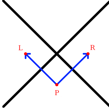
Figure 2: A source in the past, \mathcal{P} , emits an entangled photon pair that accelerates \mathcal{R} in the right Rindler wedge and \mathcal{L} in the left Rindler wedge. The two null directions of propagation define the null coordinates u = t - z + 1 and v = t + z + 1 , with the right-moving photon propagating along u = 0 and the left-moving photon along v = 0 ; these are the z^- and z^+ axes of the double-null coordinate system of Section 3.4.
