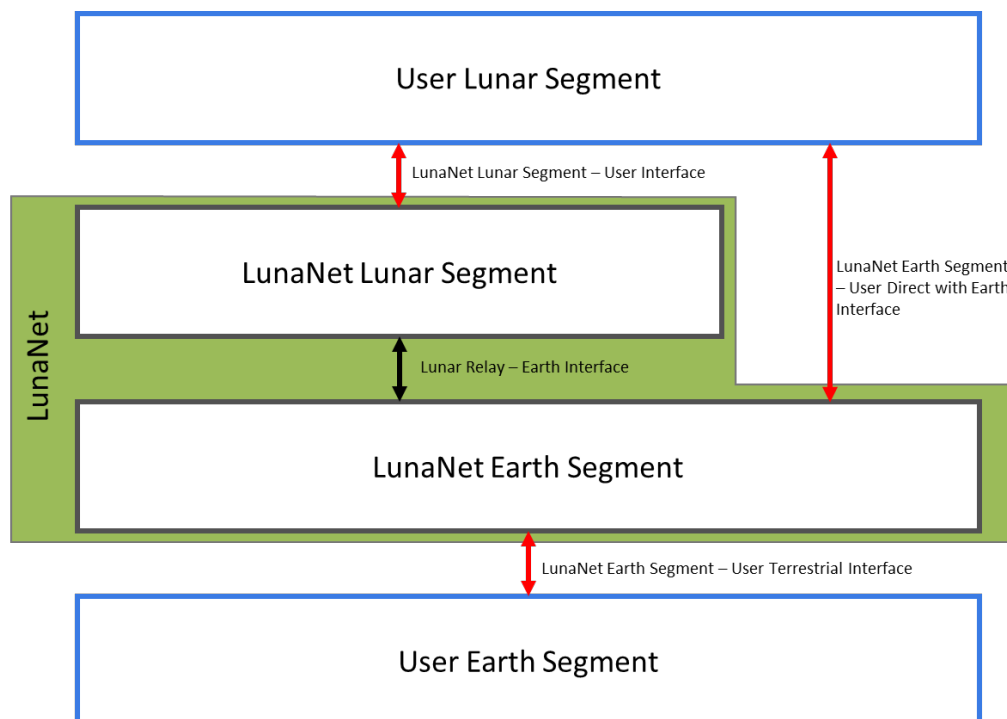
Figure 3: LunaNet Segments
