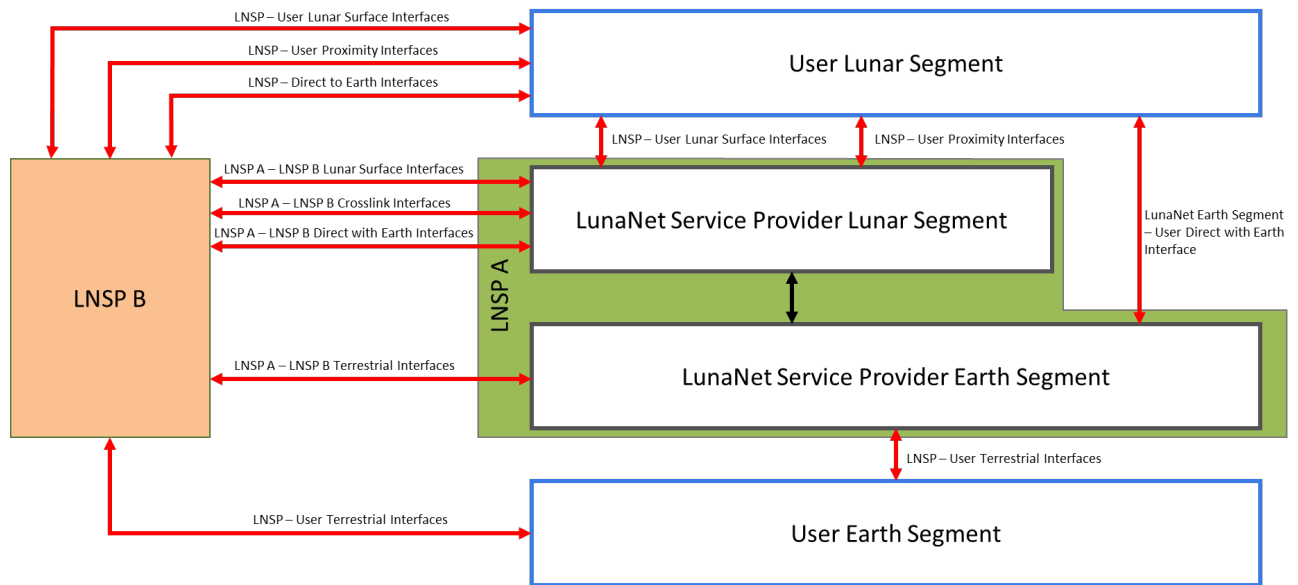
Figure 5: LunaNet Service Providers Interfaces
