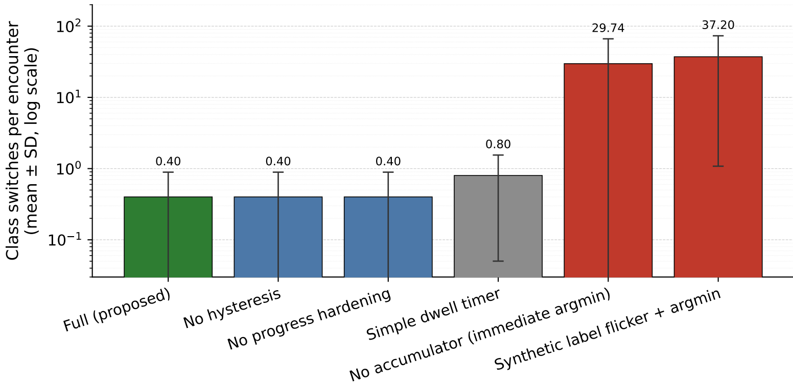
Ablations and synthetic stress comparator: label-switch count (N=250 runs/variant, 5 scenarios x 50 seeds, 10.0 s horizon)
