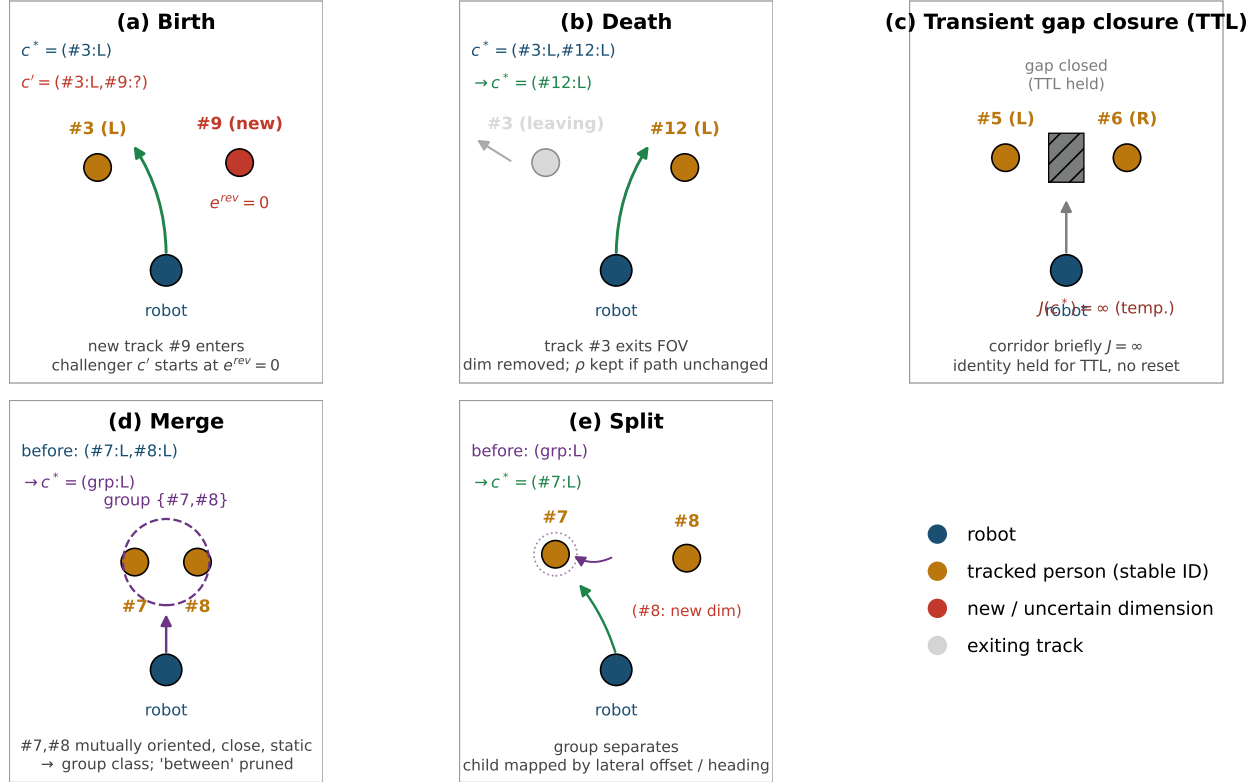
Figure 1: Schematic of the five lifecycle events of a topological class: (a) Creation — a new track appears as a challenger, starting from e^{\text{rev}} = 0 ; (b) Extinction — when a track leaves, the corresponding dimension is removed ( \rho is retained if the path is unchanged); (c) Temporary unavailability — even when a corridor momentarily becomes J = \infty , identity is retained for a TTL to prevent a reset; (d) Merge — two people judged by interaction cues (mutual orientation, proximity, low speed) merge into a single group class; (e) Split — a group separates, mapped to the child class consistent with the robot's lateral offset and heading. This emphasizes that class identity is bound to human track IDs rather than geometry.
