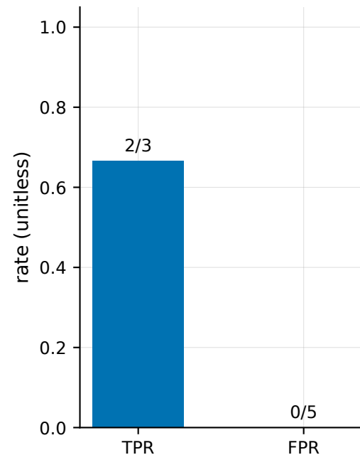
Periodic-class TPR/FPR
