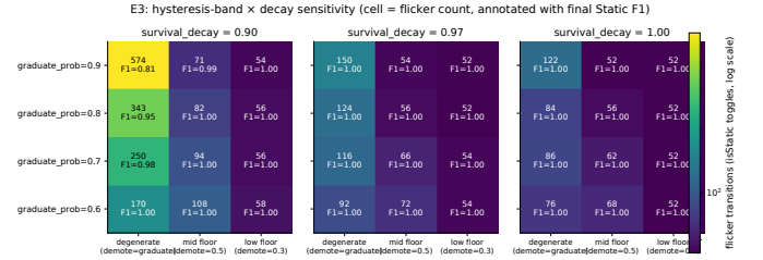
Fig. 4. E3: three heatmap panels (one per survival_decay); rows = graduate_prob, columns = hysteresis-band width, cells colored by flicker-transition count (log scale) and annotated with the raw count and final F1 — the degenerate (zero-band) column drives both the worst flicker and the worst F1 at every decay setting.
