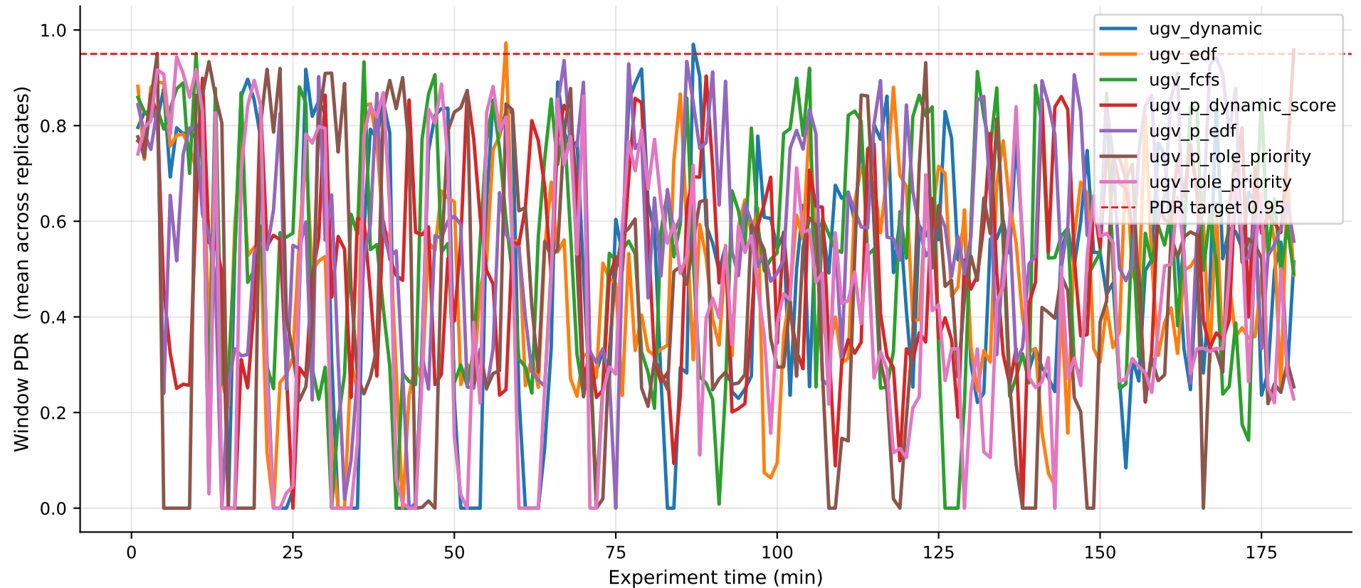
Network PDR Over Time — Merged Replicates
