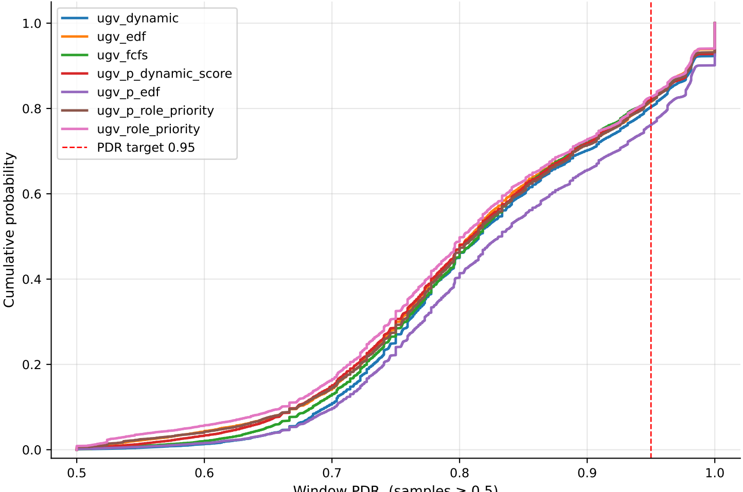
Network PDR CDF — Merged Replicates ( \text{PDR} \geq 0.5 )
