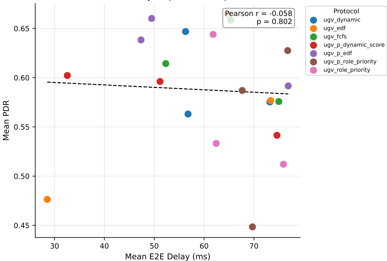
PDR vs E2E Delay — per run, all protocols
