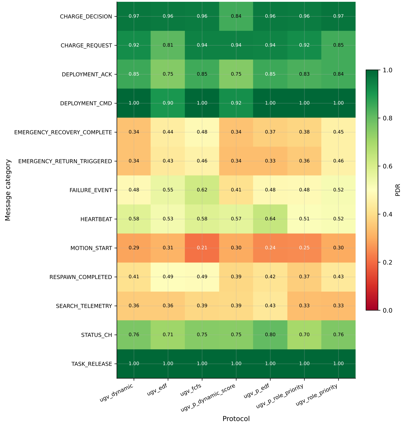
Network PDR by Message Category × Protocol — Merged Replicates
