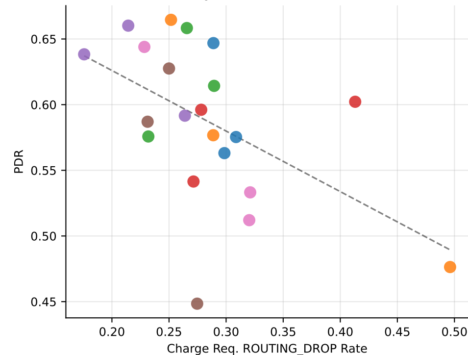
Routing Drops → Network PDR
