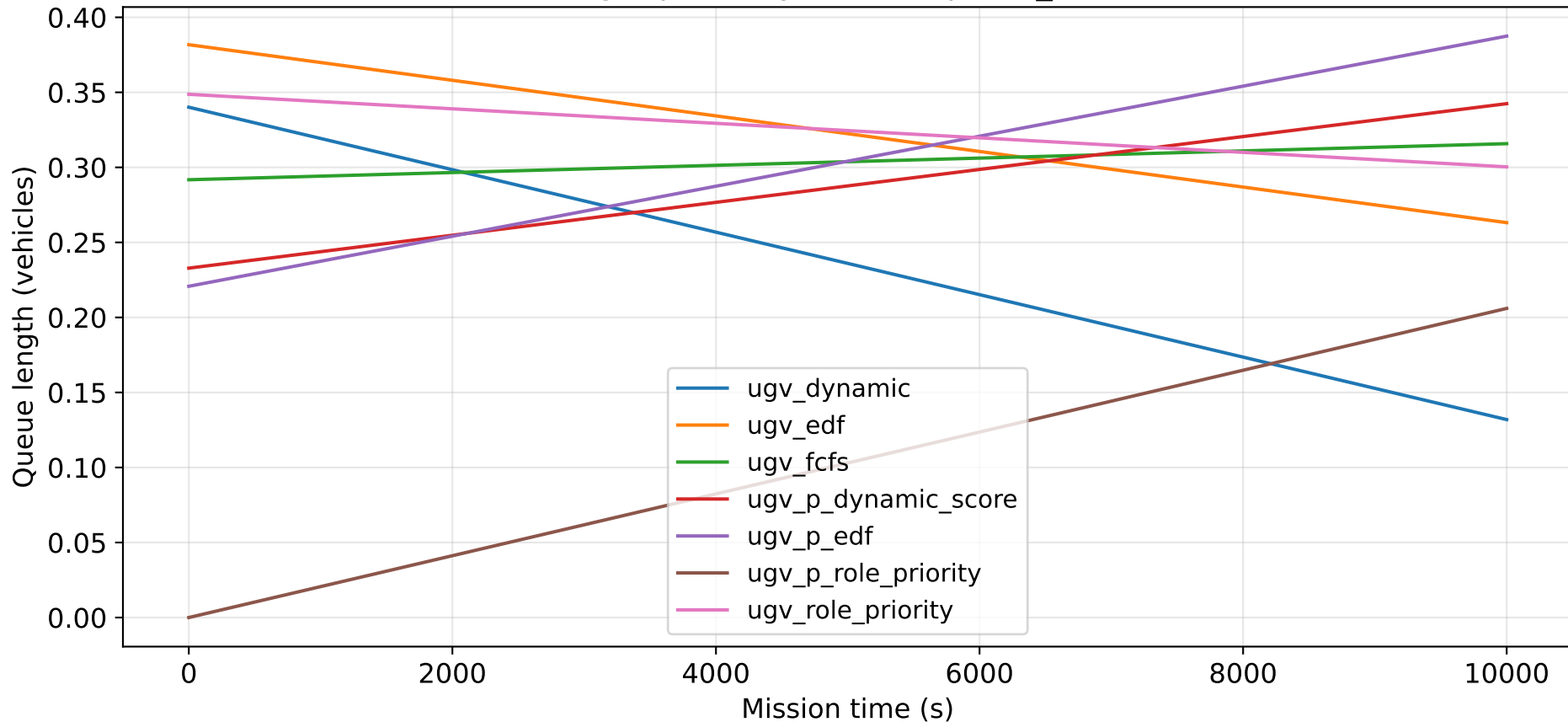
Charge queue dynamics: queue_len (all)
