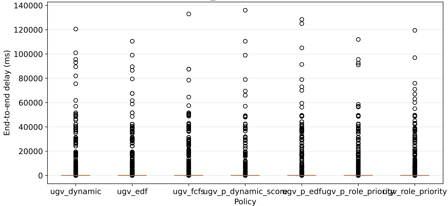
Message e2e_delay distribution by policy
