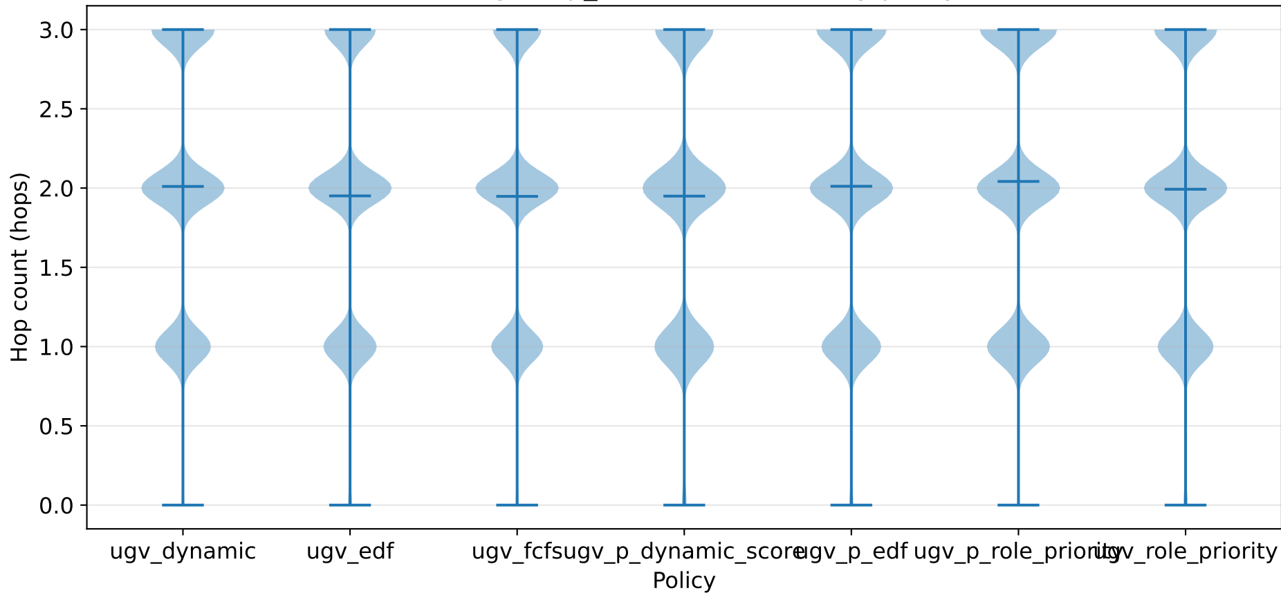
Message hop_count distribution by policy
