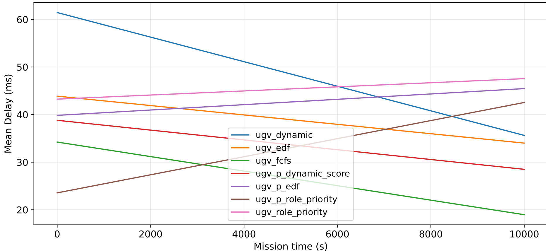
Network DELAY over mission time
