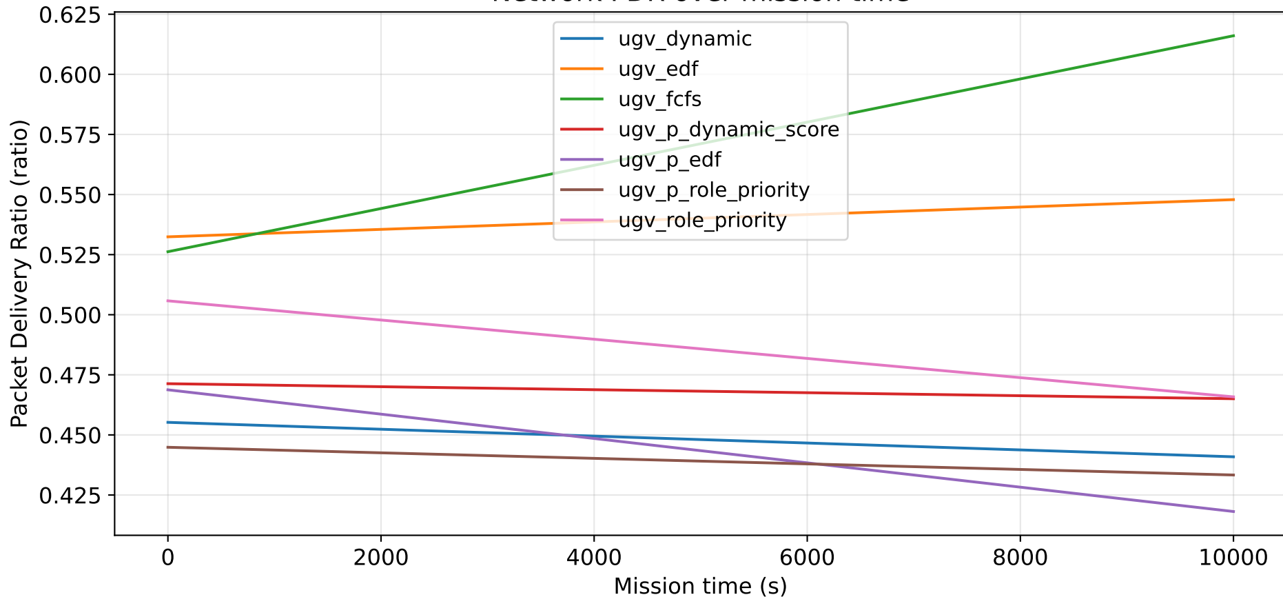
Network PDR over mission time
