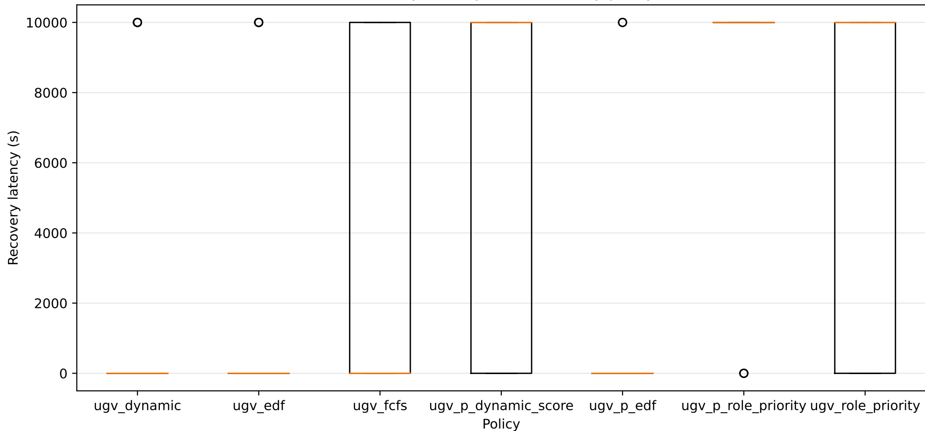
Recovery latency distribution by policy
