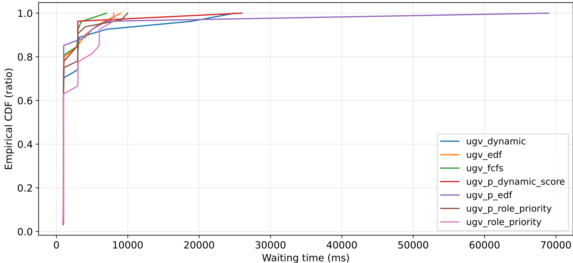
Charging wait-time CDF (CH)
