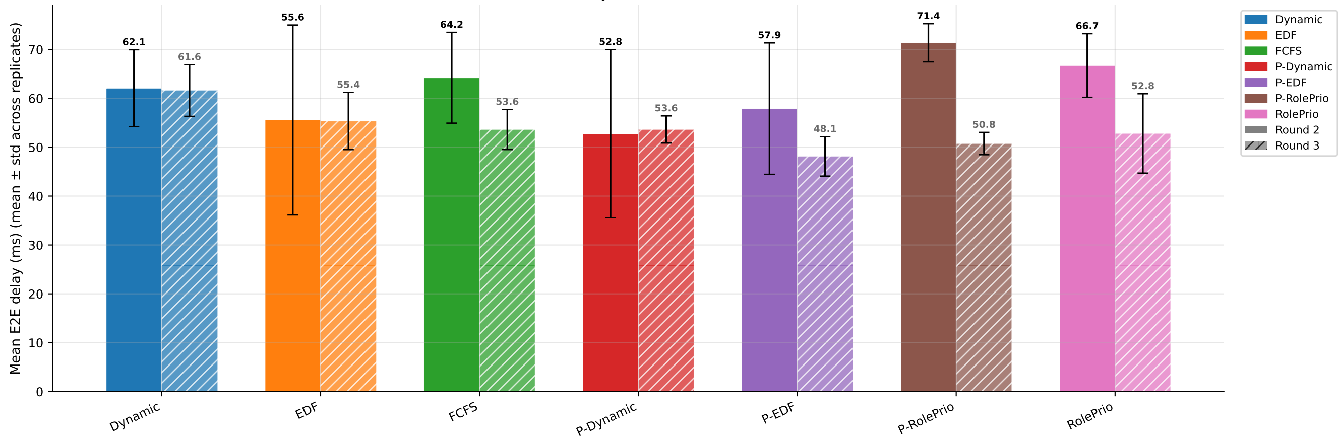
Mean E2E Delay — Round 2 vs Round 3
