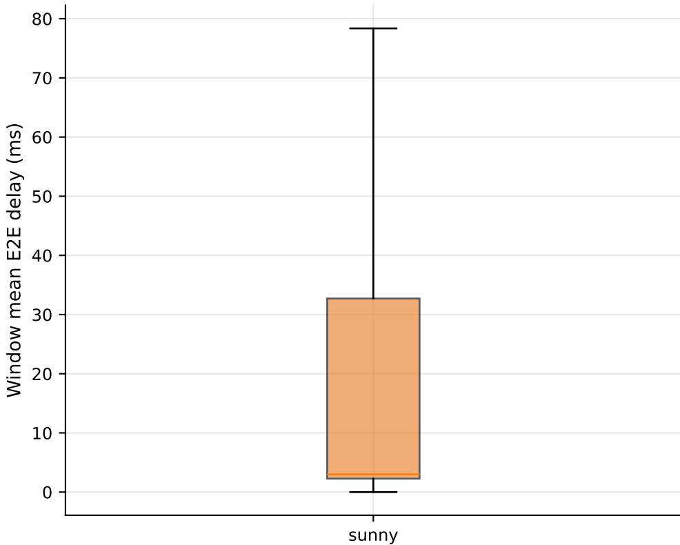
Message E2E Delay vs Weather Regime (all protocols)
