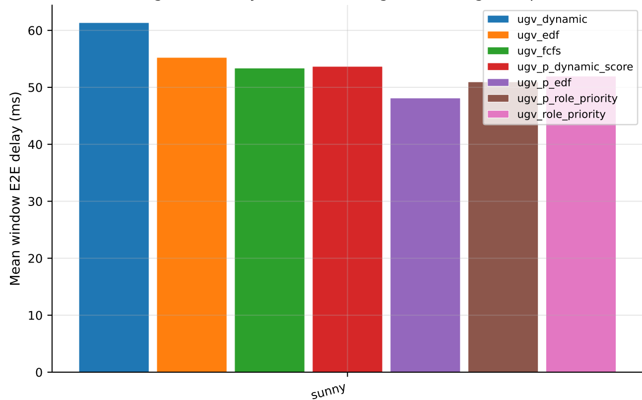
Message E2E Delay vs Weather Regime — Merged Replicates
