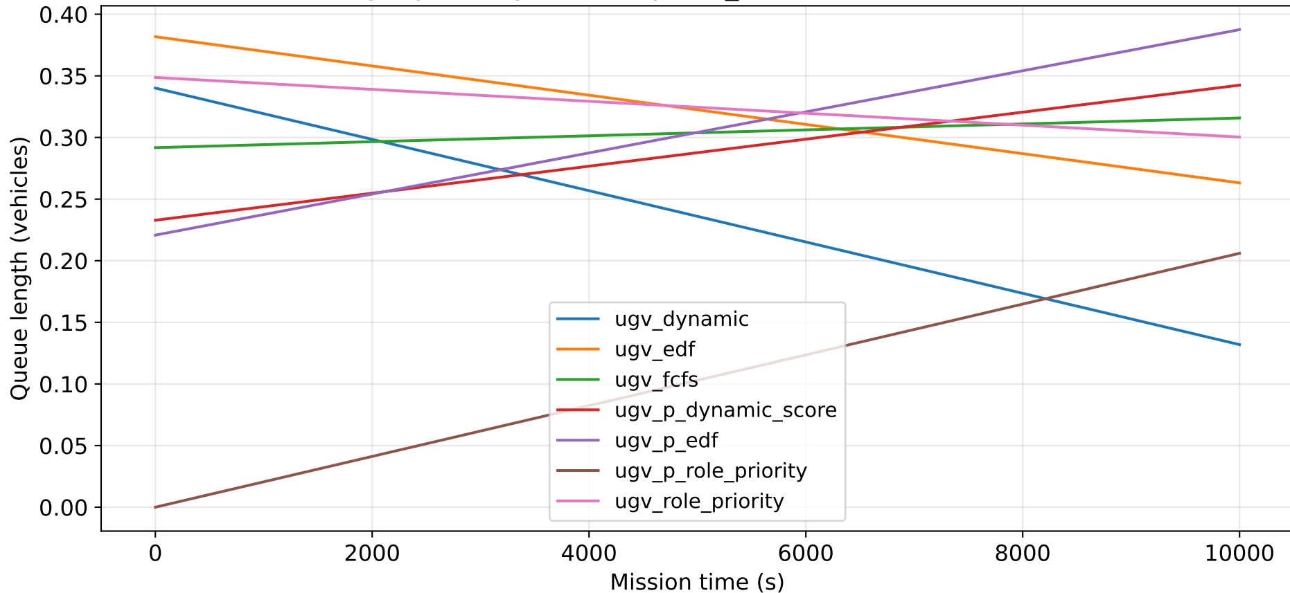
Charge queue dynamics: queue_len (all) (common window)
