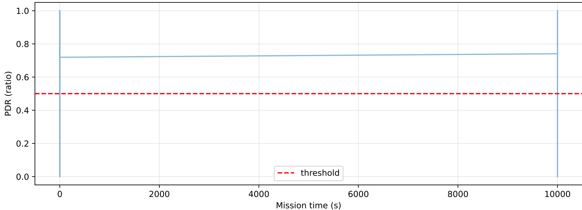
Collapse threshold PDR timeseries: ugv_dynamic (common window)
