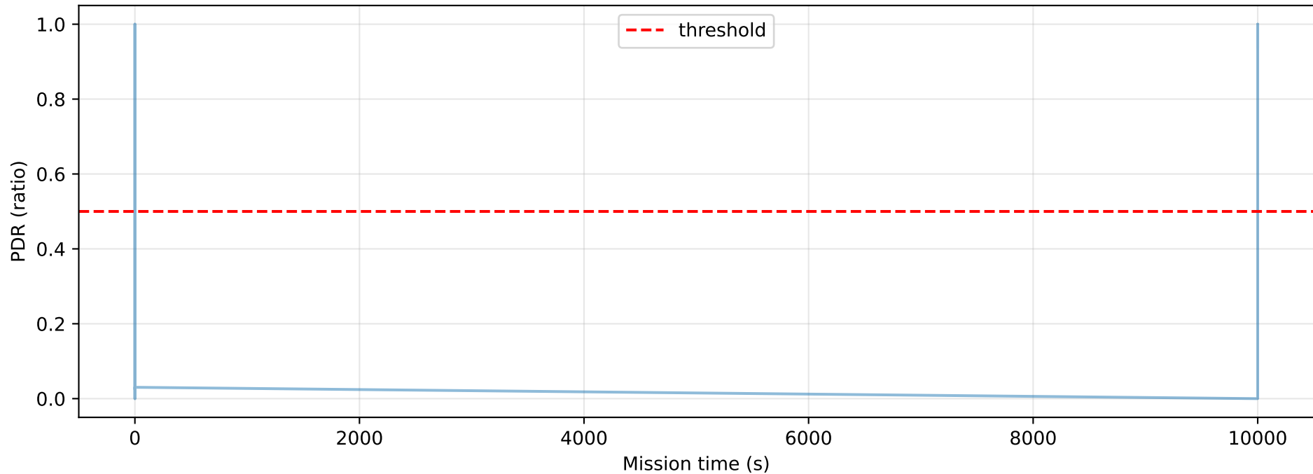
Collapse threshold PDR timeseries: ugv_edf (common window)
