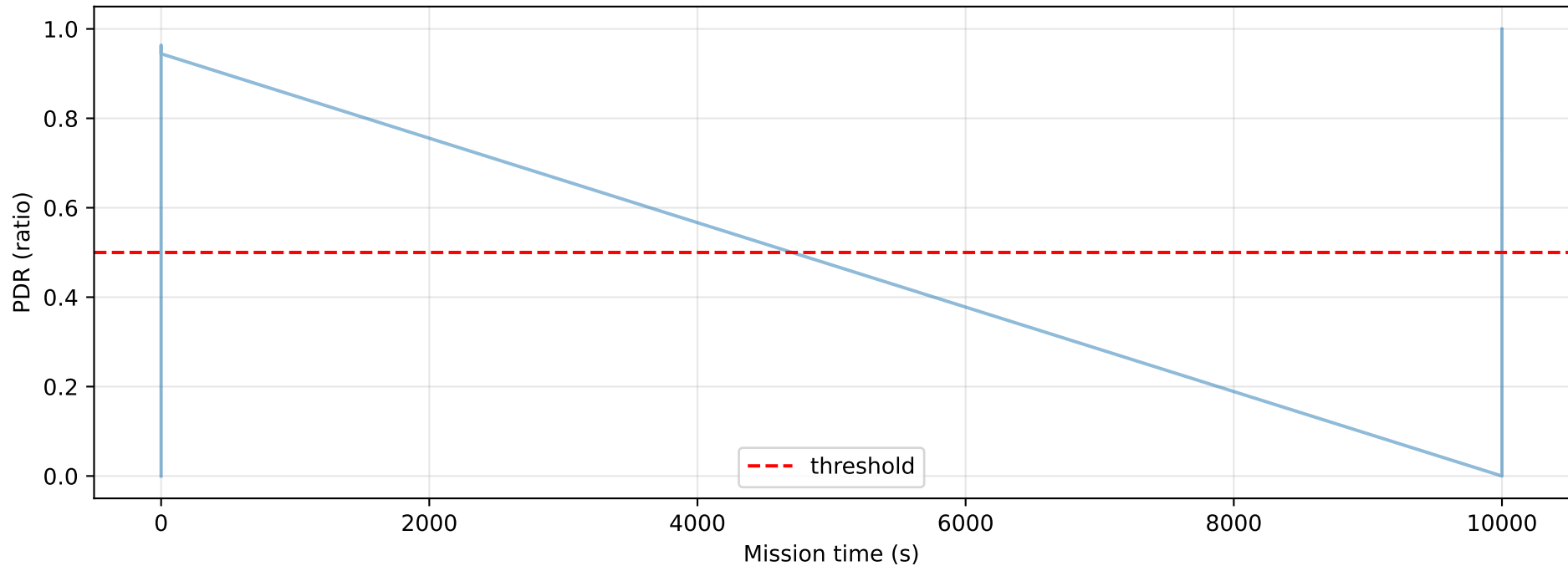
Collapse threshold PDR timeseries: ugv_p_role_priority (common window)
