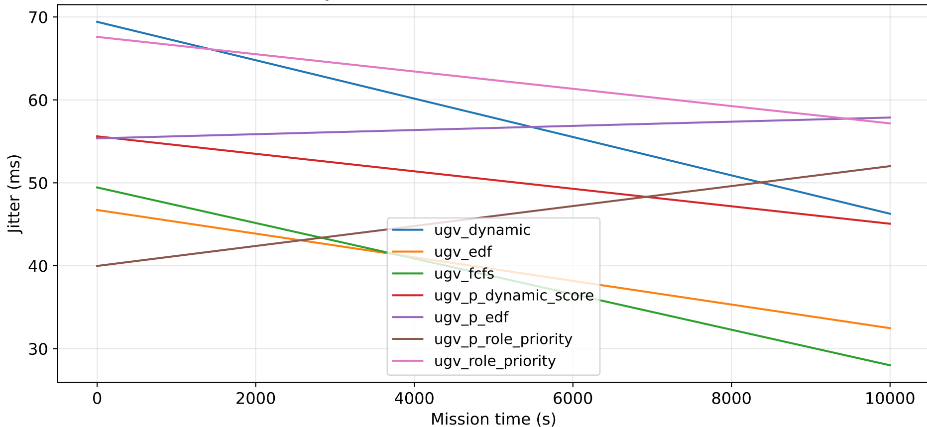
Network JITTER over mission time (common window)
