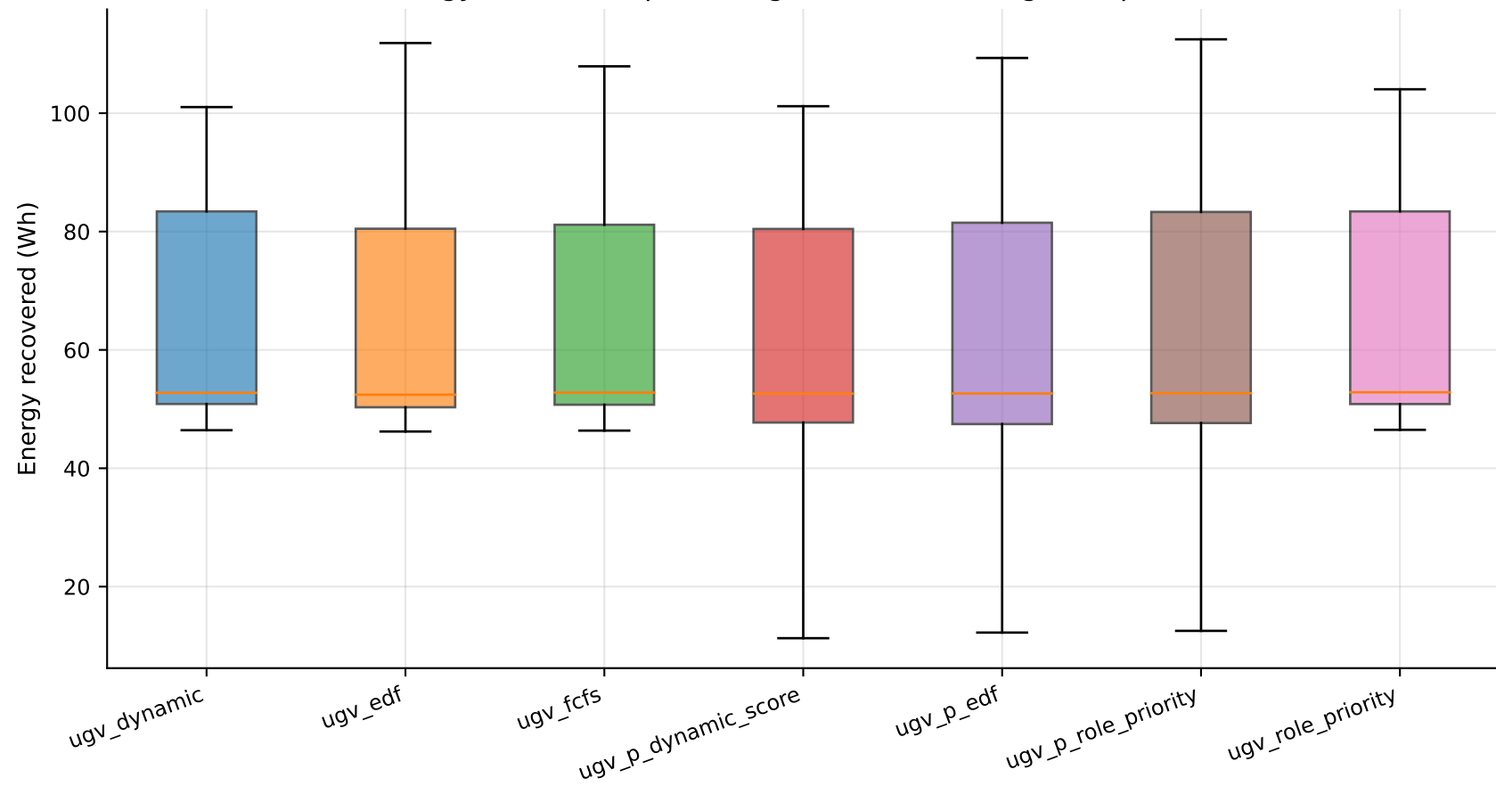
Energy Recovered per Charge Session — Merged Replicates
