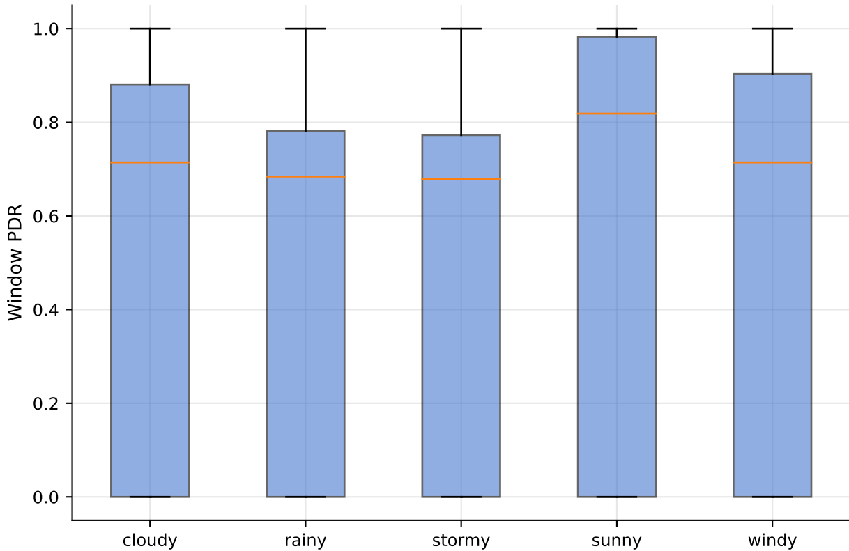
Network PDR vs Weather Regime (all protocols)
