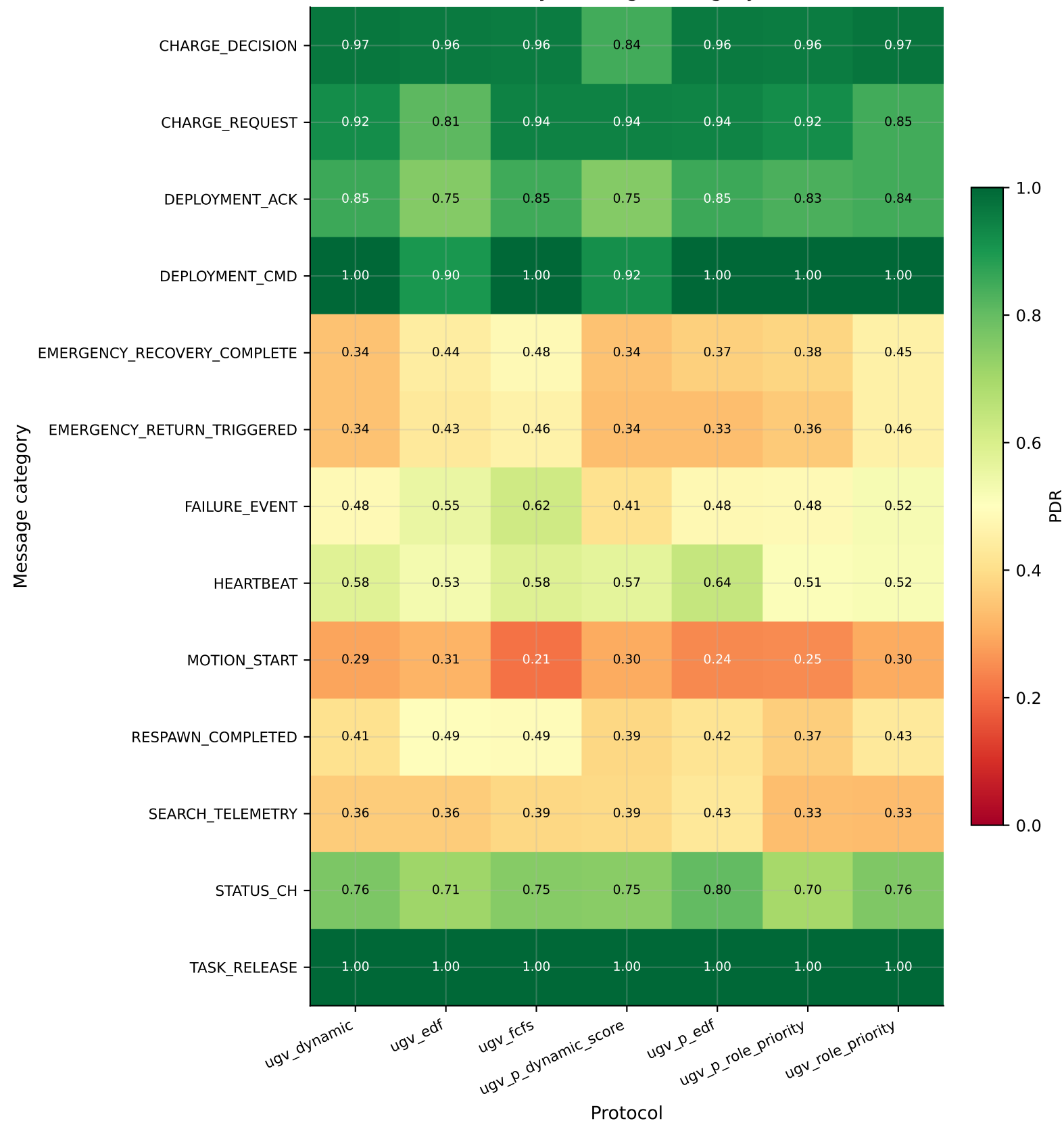
Network PDR by Message Category × Protocol
