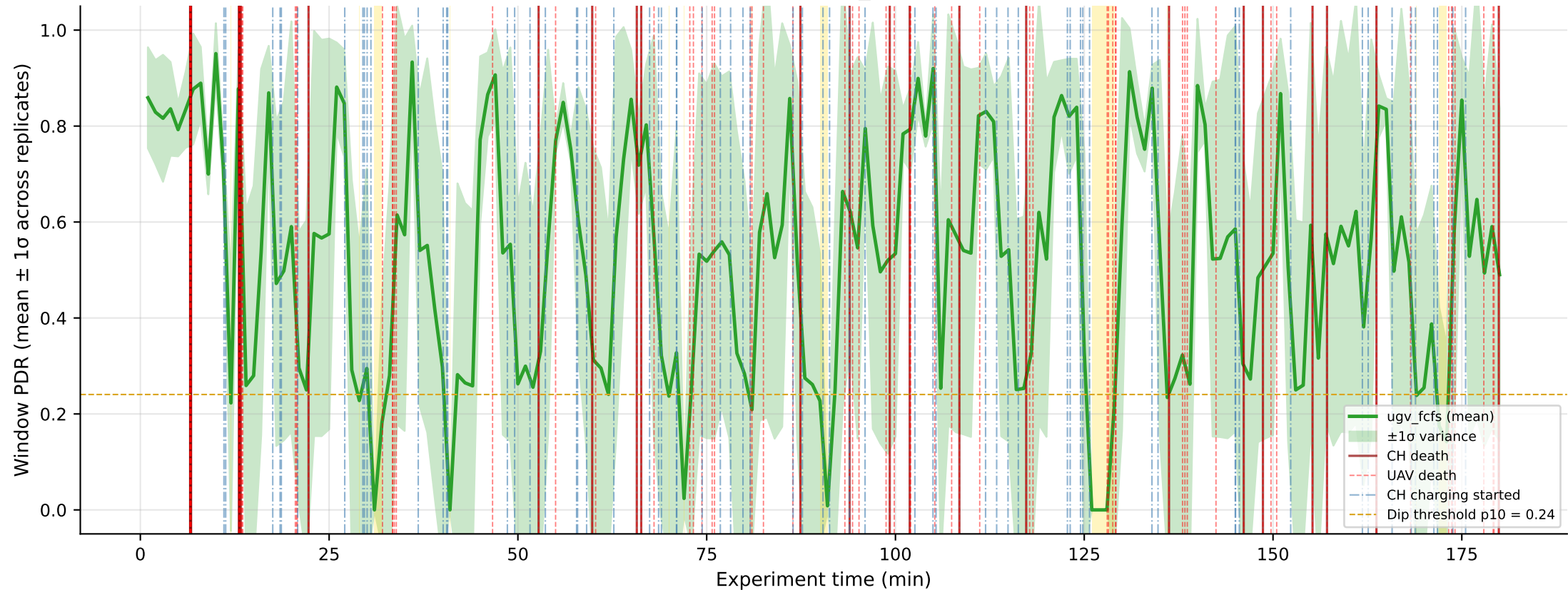
PDR + Events + Variance — ugv_fcfs — Merged Replicates
