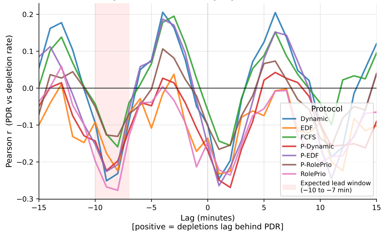
Lagged Cross-Correlation: PDR → Depletion Rate (3 replicates concatenated per protocol; 1-min bins)
