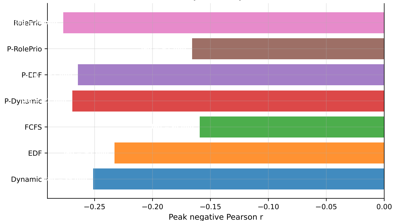
Peak Negative r & Lag (PDR drop leads depletions)
