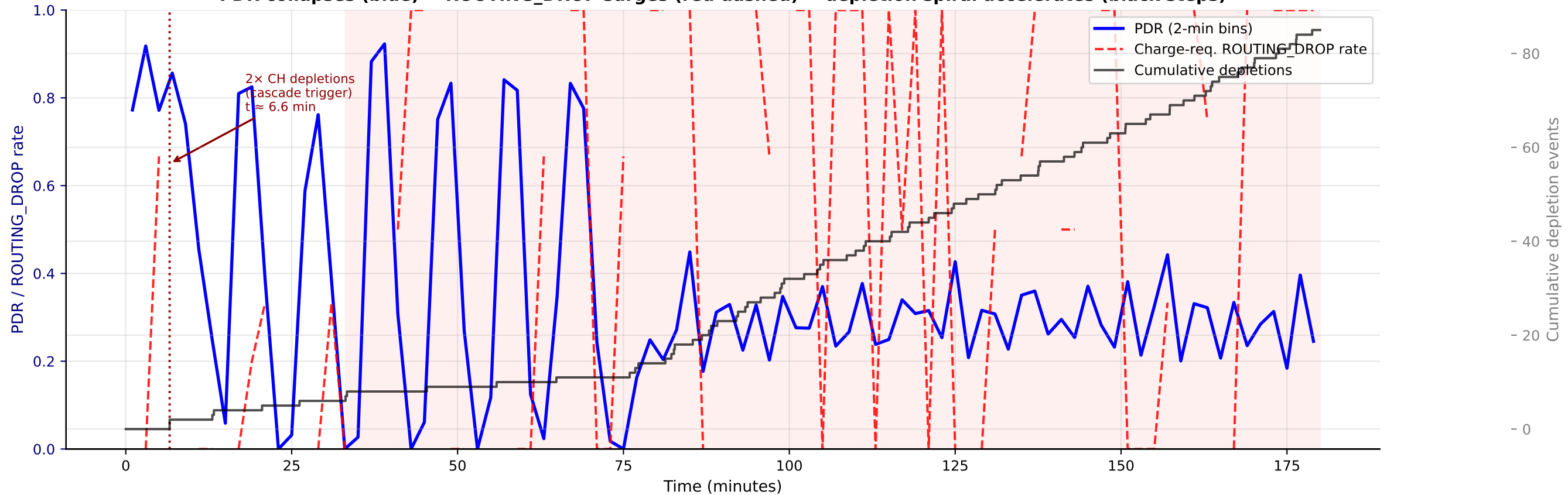
§4.4 / §5 Anomaly A — ugv_edf run 3: Cascade Failure Timeseries PDR collapses (blue) → ROUTING_DROP surges (red dashed) → depletion spiral accelerates (black steps)
